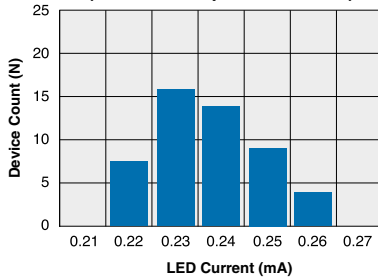
CPC1945G Typical I_F for Switch Operation (Ambient Temperature = 25°C)
