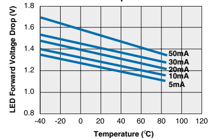
CPC1945G Typical LED Forward Voltage Drop vs. Temperature
