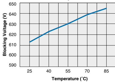
CPC1945G Typical Blocking Voltage vs. Temperature
