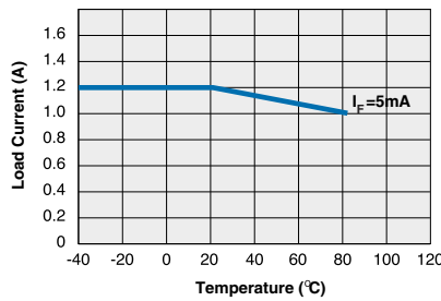
CPC1945G Typical Maximum Load Current vs. Temperature
