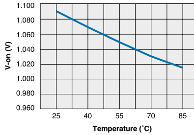
CPC1945G Typical Output V_F vs. Temperature
