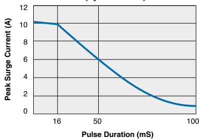
CPC1945G Maximum Surge Current (non-repetitive) ( T_J = 50^\circ\text{C max} )
