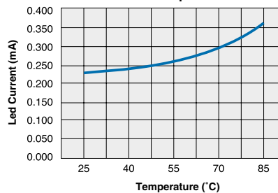
CPC1945G Typical I_F for Switch Operation Over Temperature
